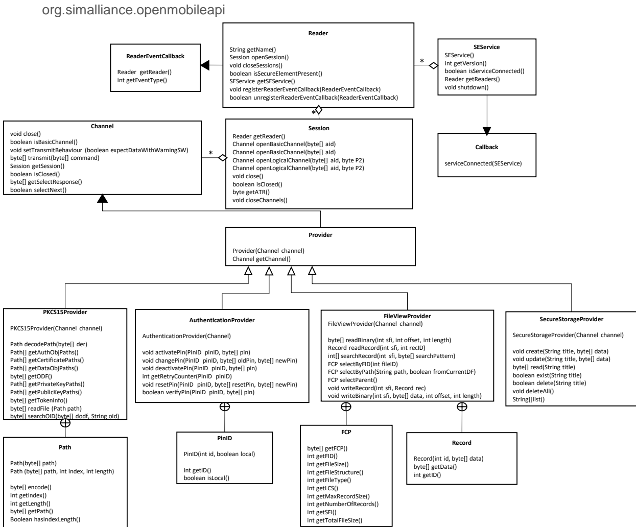
Figure 7-2: Service API class diagram with Provider classes
